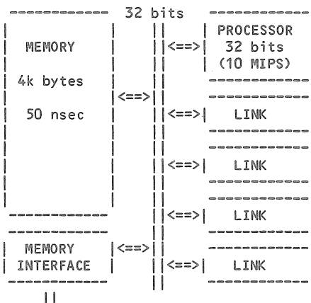
Figure 9: INMOS TRANSPUTER
