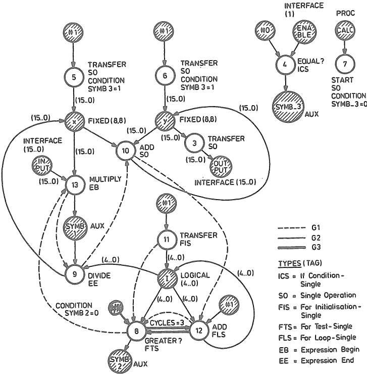
Figure 5. Internal form for exponentiation
