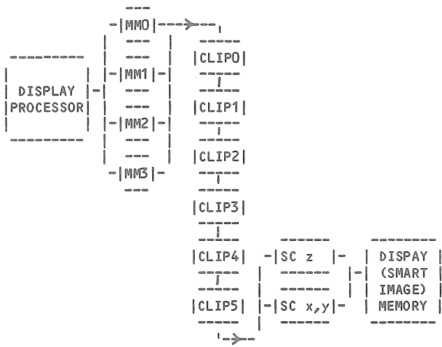
Figure 4: Geometry Engine data flow
