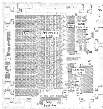
Fig. 6 Microphotograph of the digital detector
