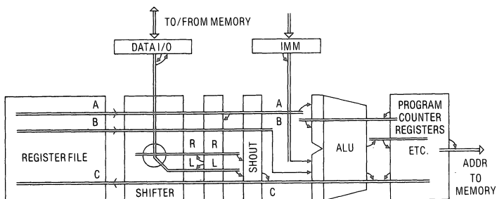
Figure 7: Berkeley RISC Microprocessors
