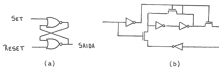
Figura 11: Flip-flops: (a) SR e (b) TOGGLE.
