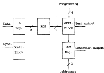
Fig. 3 Block diagram.
