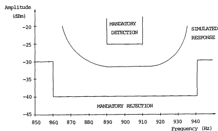
Fig. 1 Simulated response for 900 Hz detector with fixed 780 Hz tone at - 20 dBm and white gaussian noise at - 40 dBm.
