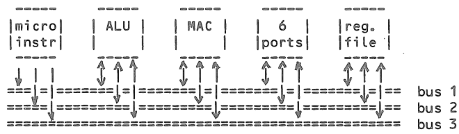
Figure 5: Programmable Systolic Chip
