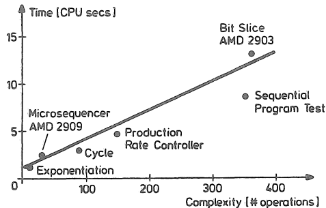
Figure 6. Time performance of the DSL compiler
