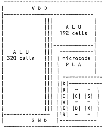
Figure 2: RSA Cipher Chip Floor Plan
