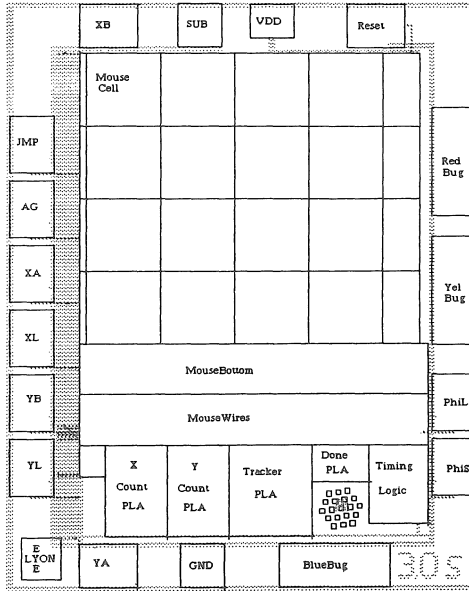
Figure 3: Optical Mouse Chip
