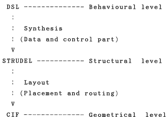
Figure 1. The DSL synthesis approach
