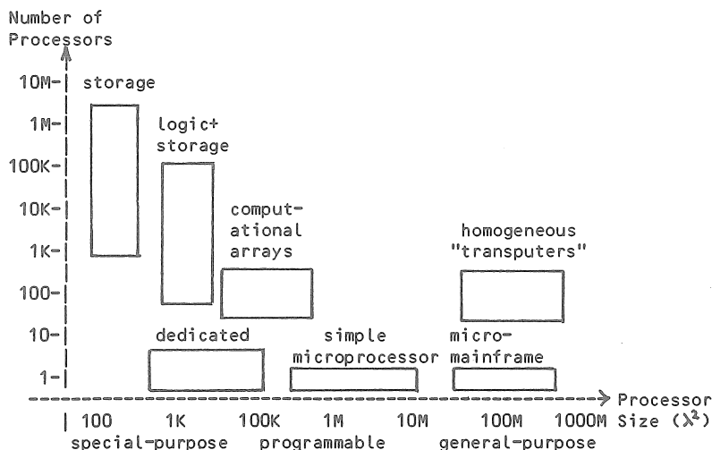
Figure 1: Taxonomy of VLSI Architectures
